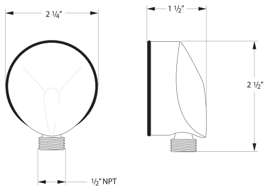
Supply elbow - P05331xx
