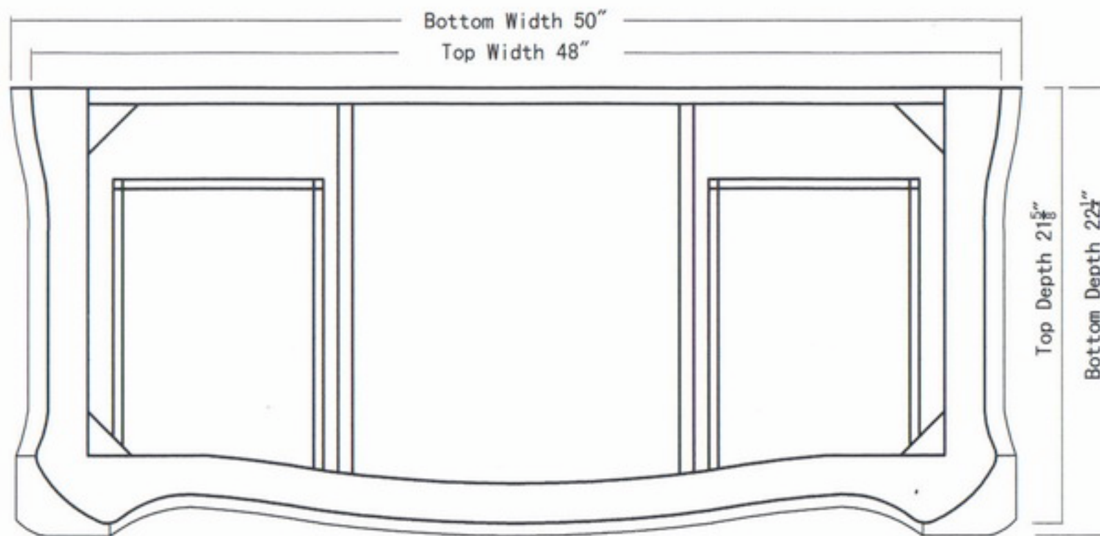
TOP VIEW
