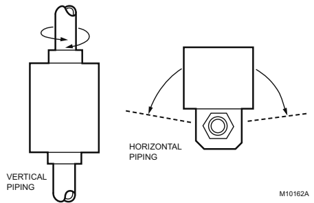
Fig. 3. Mounting positions.
