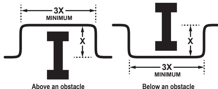
Figure 25: Installing Piping Above and Below an Obstacle.
