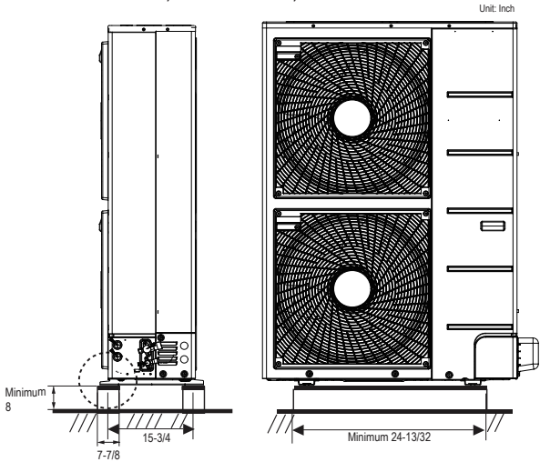
Figure 14: LMU361HHV, LMU421HHV, LMU480HHV Outdoor Units.
