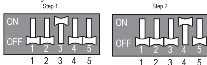
Figure 118: LMU361-421-480HHV Reducing Power Consumption DIP Switch Settings.
