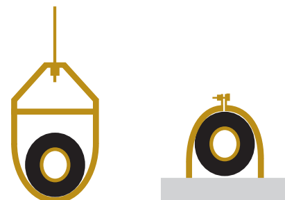
Figure 26: Pipe Hanger Details.
