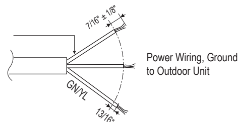
Figure 77: Multi F / Multi F MAX with LGRED Outdoor Unit Power Wiring.
