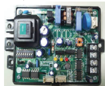
Figure 90: PI-485 Board (Appearance will differ depending on model).
