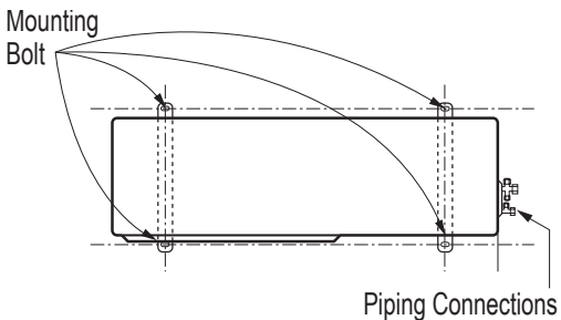
Figure 15: Bolting the Outdoor Unit to the Platform (Piping Location Will Differ Depending on Outdoor Unit Model).
