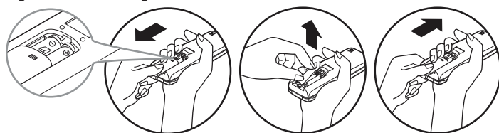
Figure 106: Installing the Remote Controller Batteries.
