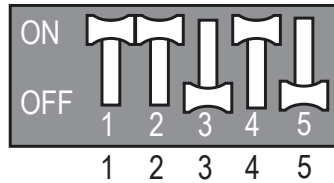
Figure 120: LMU361-421-480HHV Saving Power Consumption with Mode Lock DIP Switch Settings.
