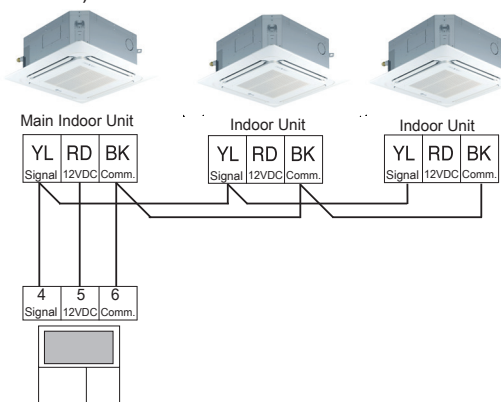
Figure 95: Example of Indoor Unit Group to Zone Controller Connections (CN-REMO).
