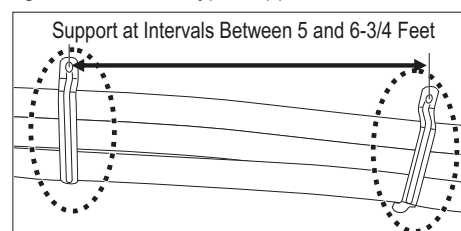
Figure 33: Saddle-Type Support.
