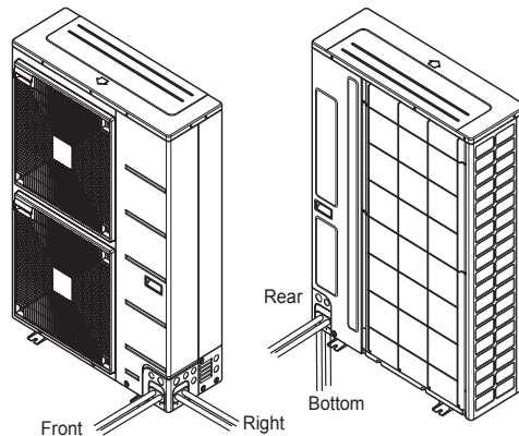
Figure 46: Multi F MAX with LGRED Outdoor Unit Refrigerant Piping Connection Options.
