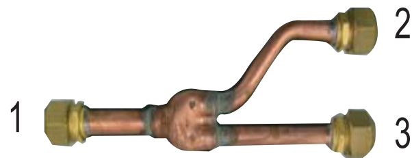
Figure 56: Y-Branch Port Identifier Diagram.
