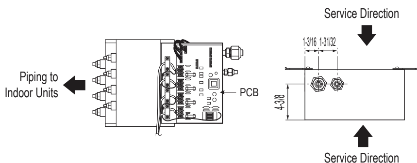
Figure 10: Branch Distribution Unit Key Components.
