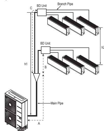
Figure 23: Multi F MAX Refrigerant Piping System Limitations.
