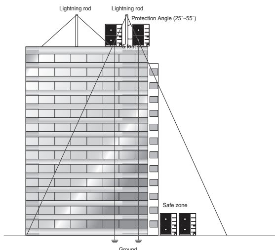
Figure 4: Lightning Protection Diagram.
