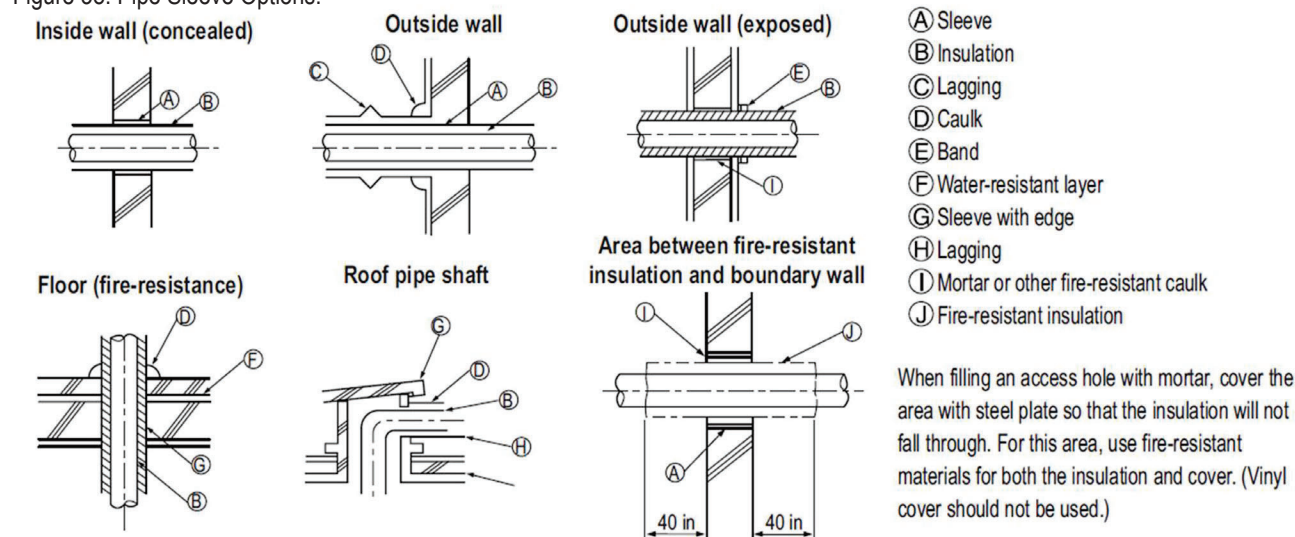
Figure 38: Pipe Sleeve Options.
