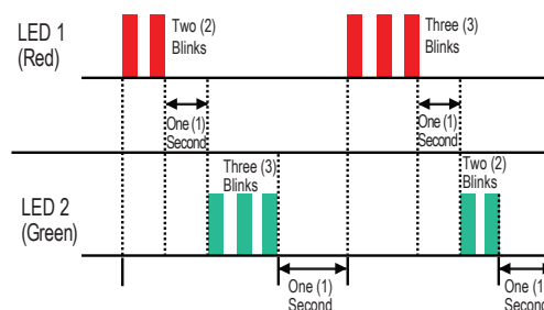
Figure 115: Wiring Error Check Example.
