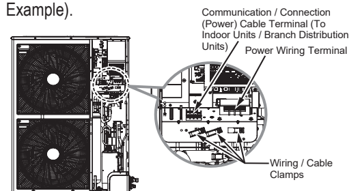
Figure 70: Location of the Power Wiring and Communication Cable Terminals (LMU361-421-480HHV Example).
