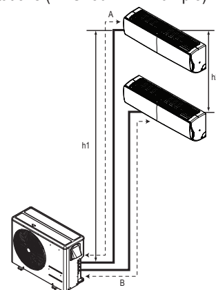
Figure 22: Multi F Refrigerant Piping System Limitations (LMU180HHV Example).
