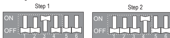
Figure 118: LMU361-421-480HHV Reducing Power Consumption DIP Switch Settings.
