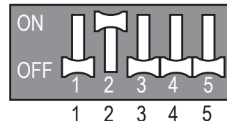
Figure 114: LMU361-421-480HHV Wiring Error Check Example.
