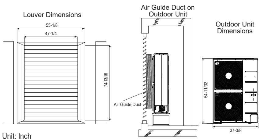
Figure 9: Example of Installing Outdoor Unit Indoors.
