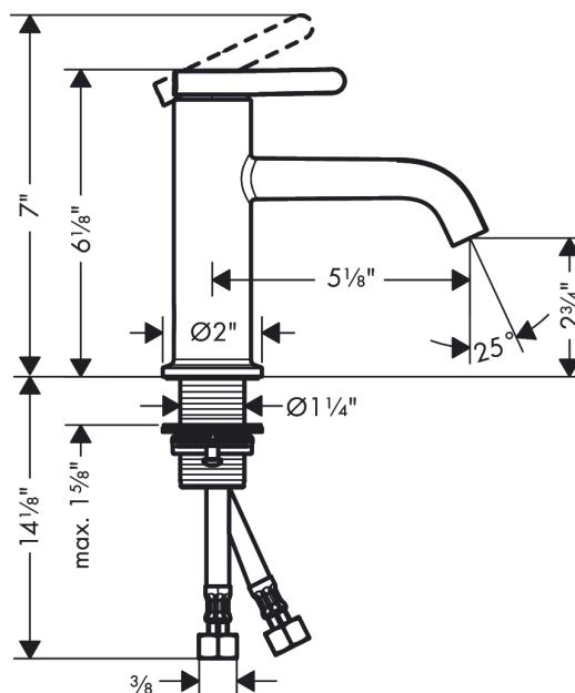
Scale drawing
