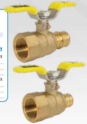
FULL PORT FORGED BRASS BALL VALVE w/ Reversible Handle & Adjustable Packing Gland
