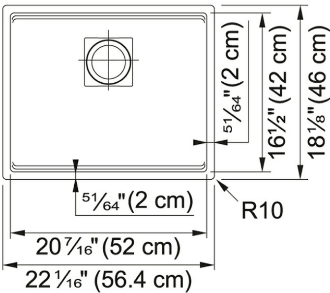
Technical Drawing
