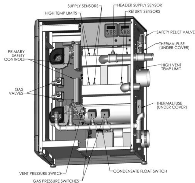
Figure 3: Control & Safety Device Locations – PF-850/1000/1500
