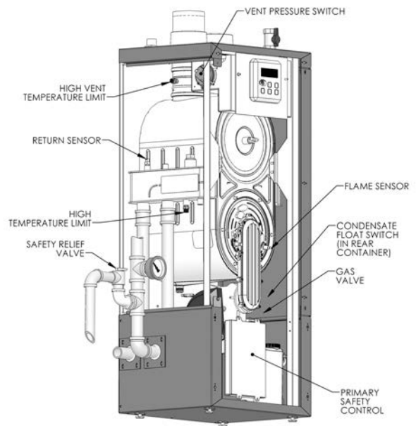
Figure 2: Control & Safety Device Locations – PF-210/399
